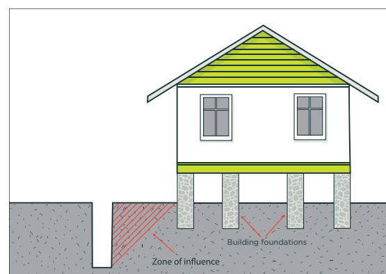
Figure 10: Building line restriction
