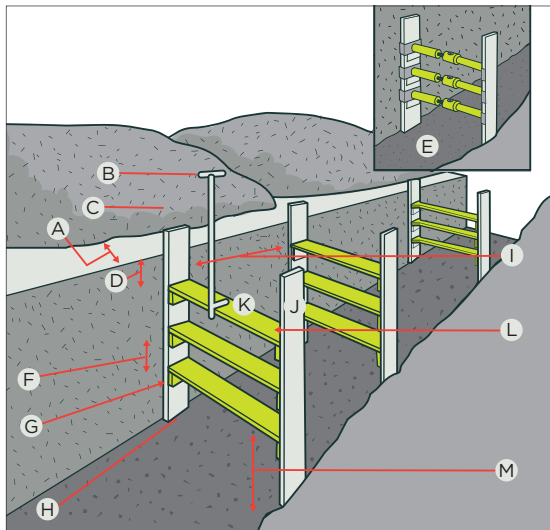
Figure 35: Soldier sets
