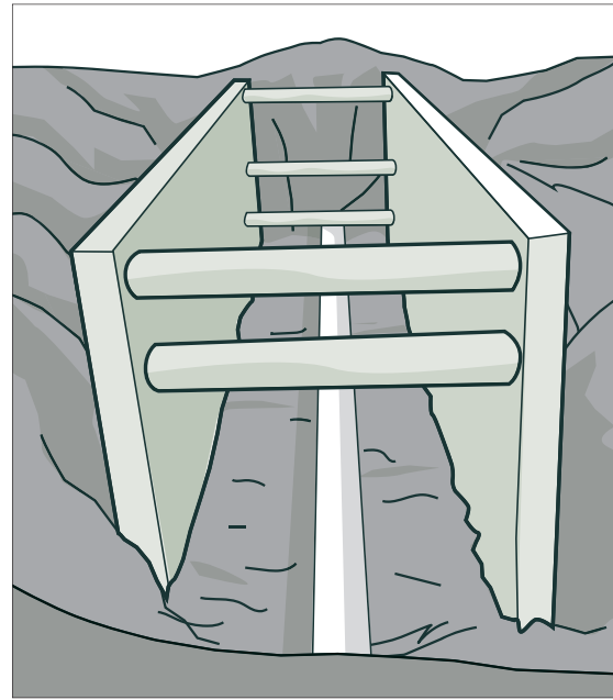
Figure 4: Trench
